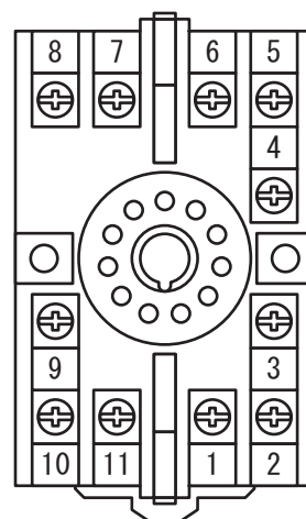
SOCKET TOP VIEW
